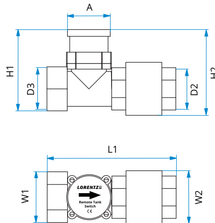
Without adapters for pipe size 1-1/2"
